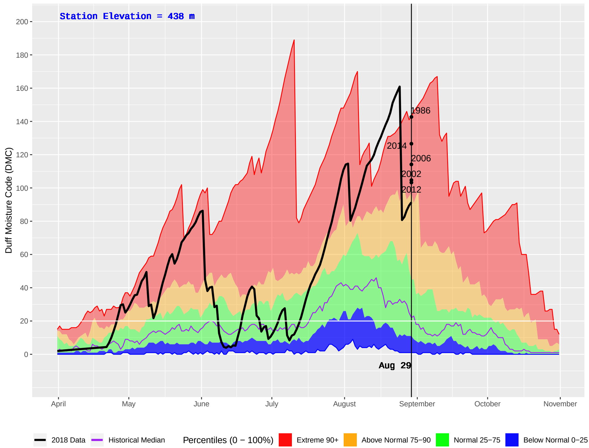
MENZIES CAMP (19) : Historical (1970–2016) and Current (2018) Daily Duff Moisture Code (DMC)
